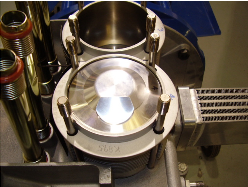
1925cc Twin Plug Test 4 vs. Test 5
