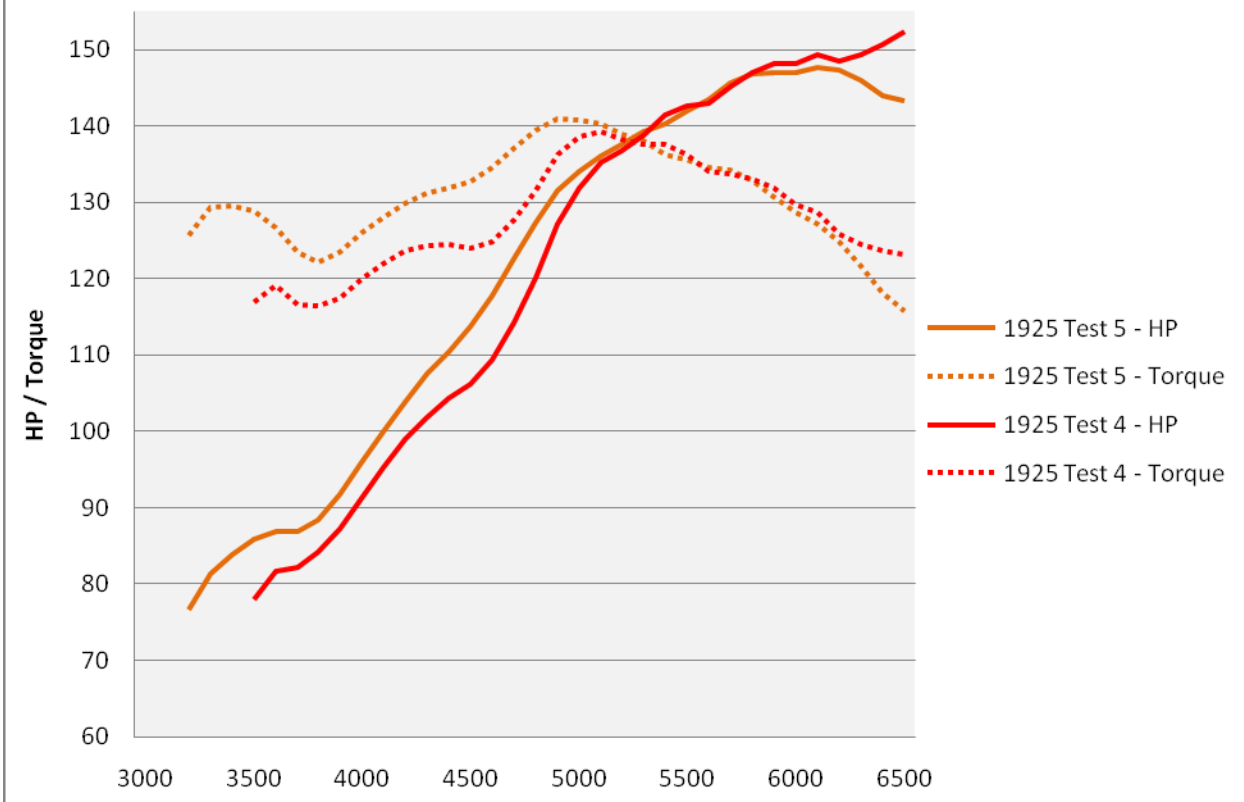
1925cc Twin Plug Test 4 vs. Test 5
